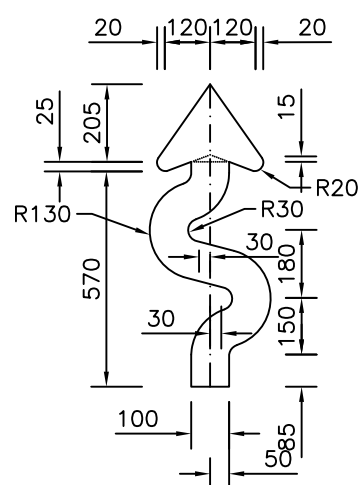
ARROW DETAILS
